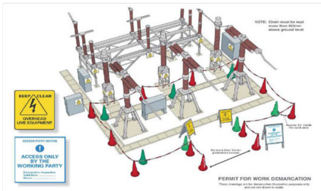
Example of a National Grid NSI 6 Demarcation Layout for Substation Work Areas
